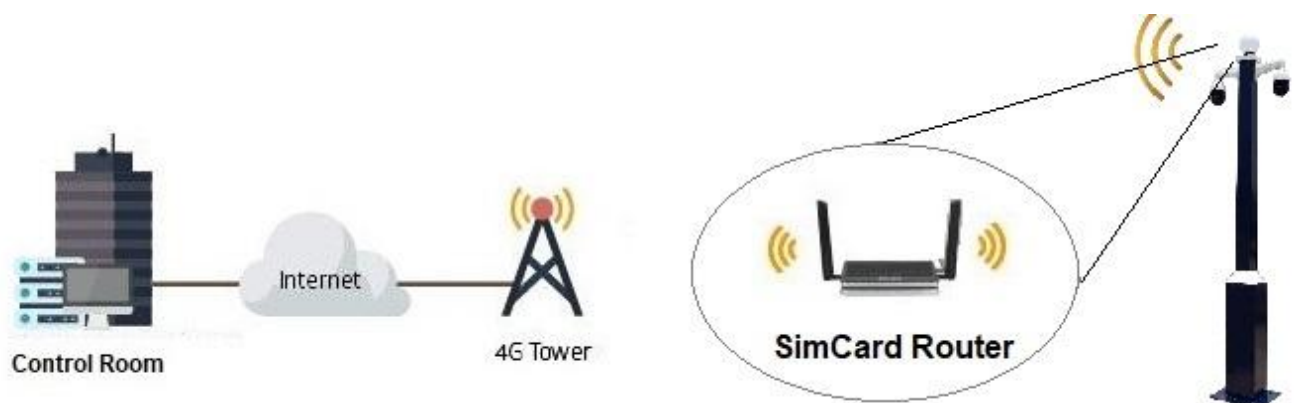
Picture 7: Data transferring with Simcard Router
